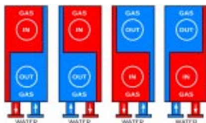
▲ Typical Plate-Fin Construction
